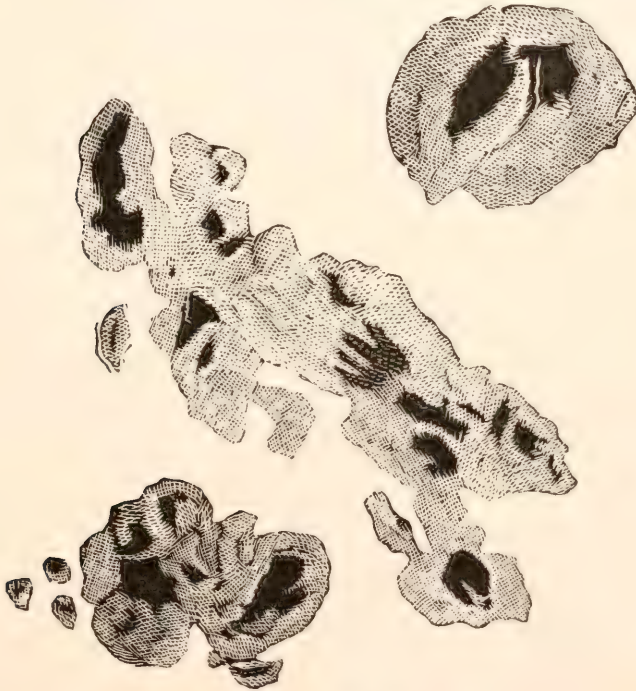
257. Spots on the Sun.
